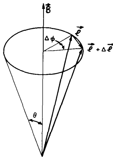
Figure 14.2. In a small time \Delta t , the tip of the \mathbf{l} vector precesses by an angle \Delta\phi around the magnetic field vector.
