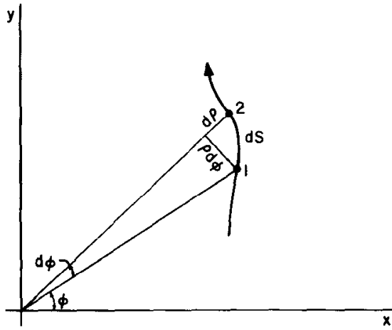
Figure 2.3. Points (1) and (2) are positions of the particle at times differing by \Delta t .
