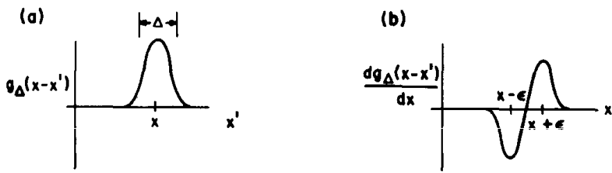
Figure 1.8. (a) The Gaussian g_{\Delta} approaches the delta function as \Delta \rightarrow 0 . (b) Its derivative (dg/dx)(x-x') approaches \delta'(x-x') as \Delta \rightarrow 0 .
