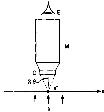
Figure 4.3. Light of frequency \lambda bounces off the electron, enters the objective O of the microscope ( M ) and enters the eye E of the observer.
