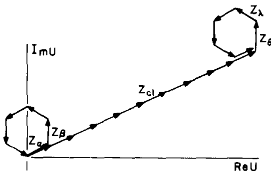
Figure 8.2. Schematic representation of the sum \Sigma . Paths near x_{cl}(t) contribute coherently since S is stationary there, while others cancel each other out and may be ignored in the first approximation when we calculate U(t) .
