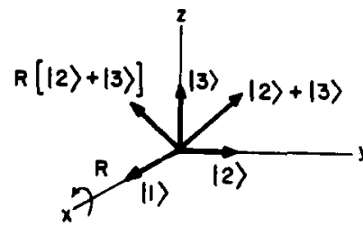
Figure 1.3. Action of the operator R(\frac{1}{2}\pi\mathbf{i}) . Note that R[|2\rangle+|3\rangle]=R|2\rangle+R|3\rangle as expected of a linear operator. (We will often refer to R(\frac{1}{2}\pi\mathbf{i}) as R if no confusion is likely.)
